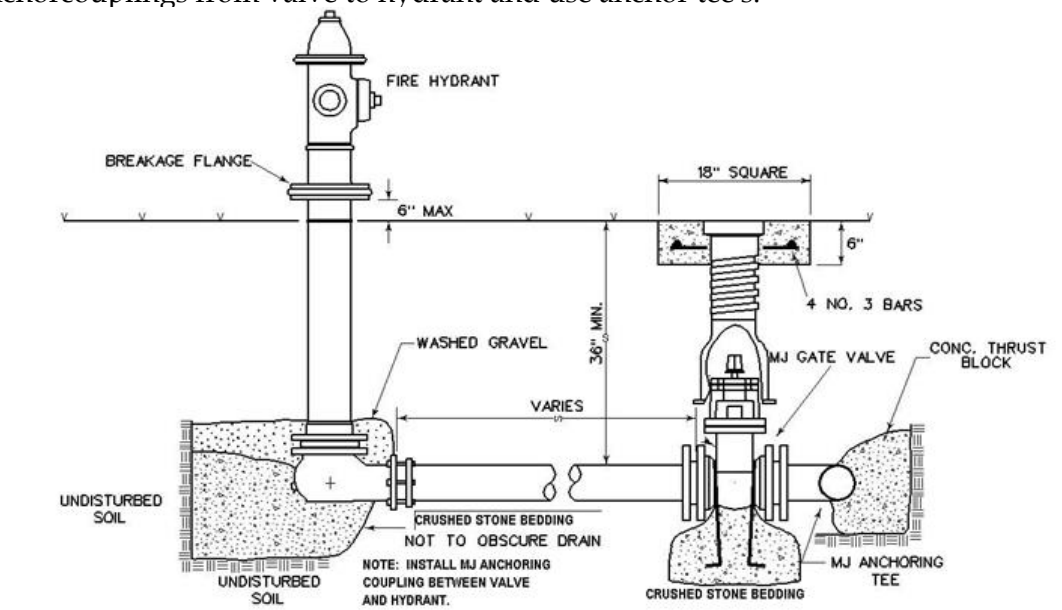
ILLUSTRATION 3.4.2. – FIRE HYDRANT INSTALLATION
